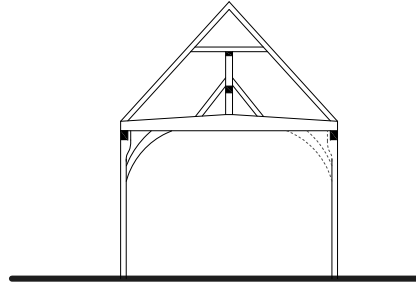
Figure 2b Section A-A
